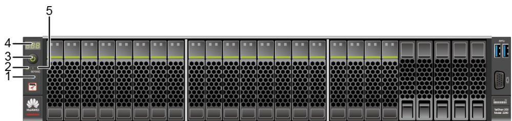
图 2-8 8x2.5 SAS/SATA+12x2.5 NVMe 硬盘配置前面板指示灯和按钮
