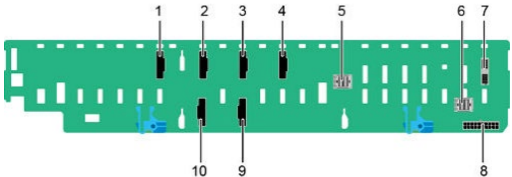
图 2-27 8x2.5 SAS/SATA+12x2.5 NVMe 硬盘背板( Part No.: 03029TDE)
